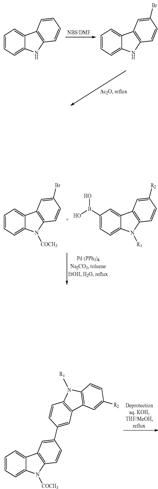
Scheme 8: Synthesis of compounds from 6-1 to 6-6
