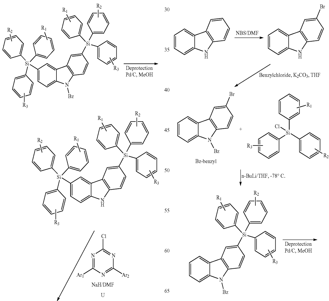
Scheme 10: Synthesis of compounds from 7-6 to 7-10
