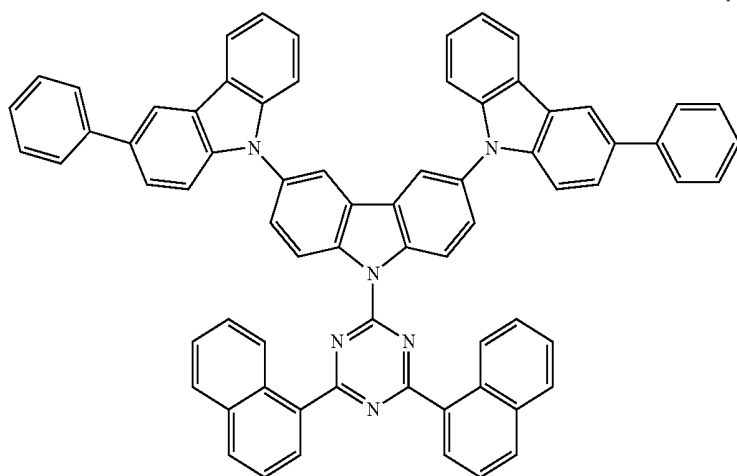
Compound 1-25
