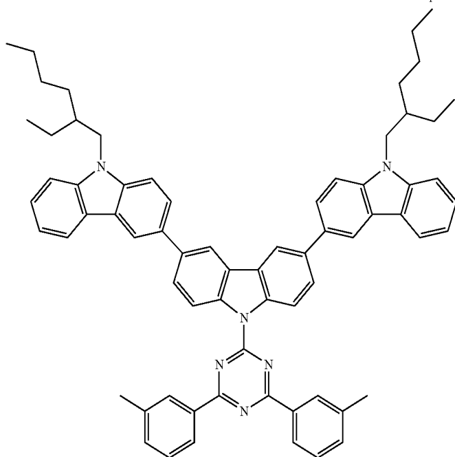
Compound 5-6
