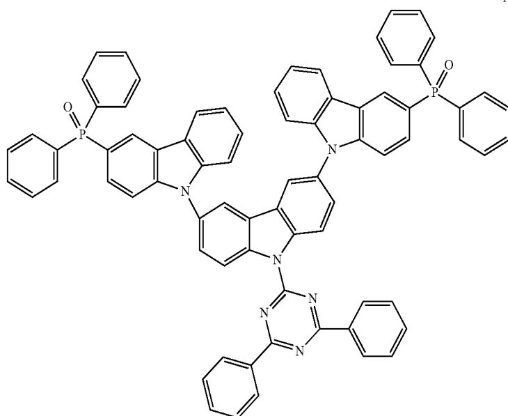
Compound 1-50
