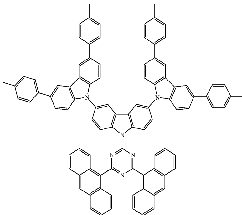
Compound 1-44
