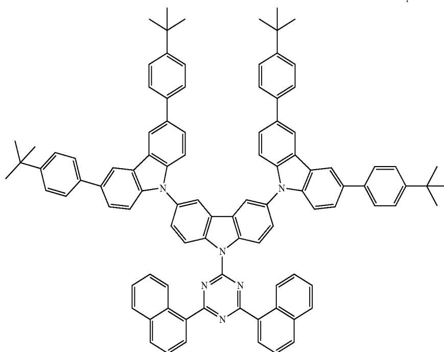
Compound 1-28
