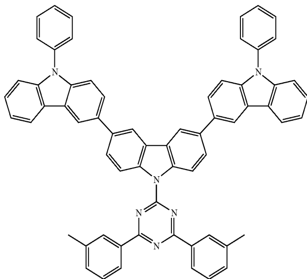
Compound 5-7
