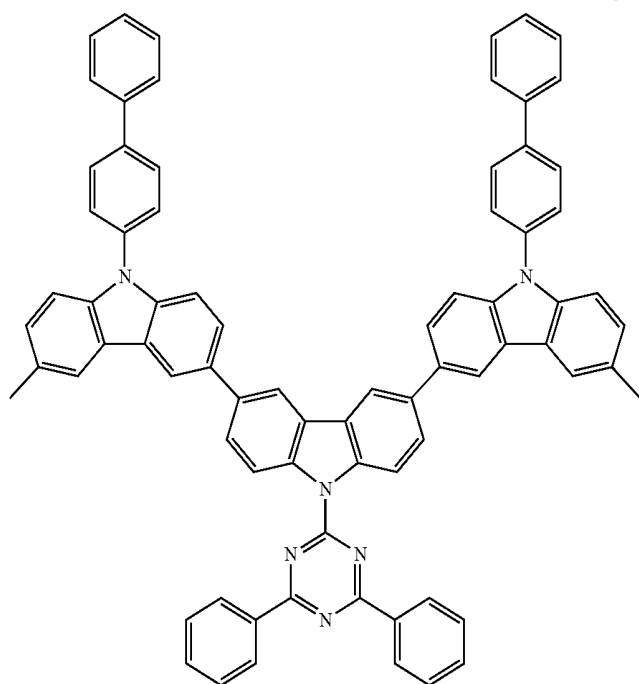
Compound 5-4
