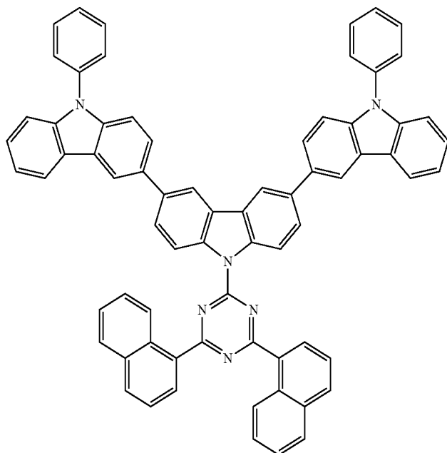
Compound 5-9
