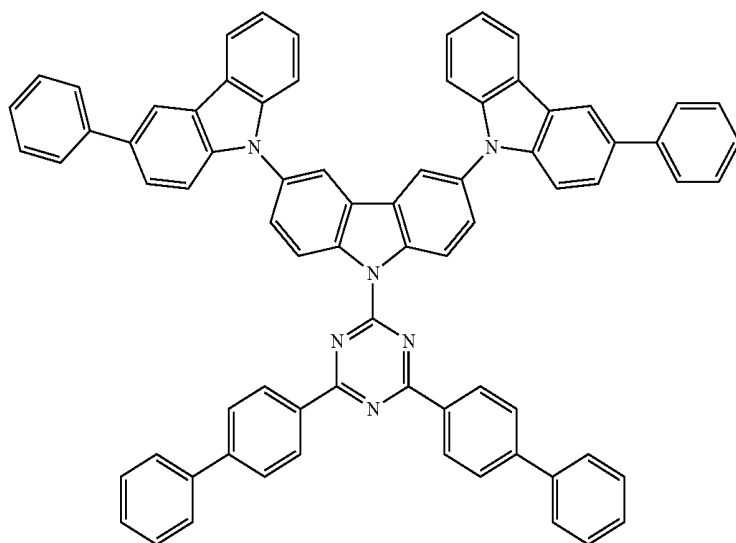
Compound 1-35
