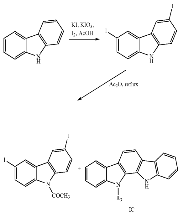
Scheme 3: Synthesis of compounds from 3-1 to 3-7
