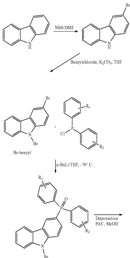
Scheme 12: Synthesis of compounds from 8-8 to 8-12
