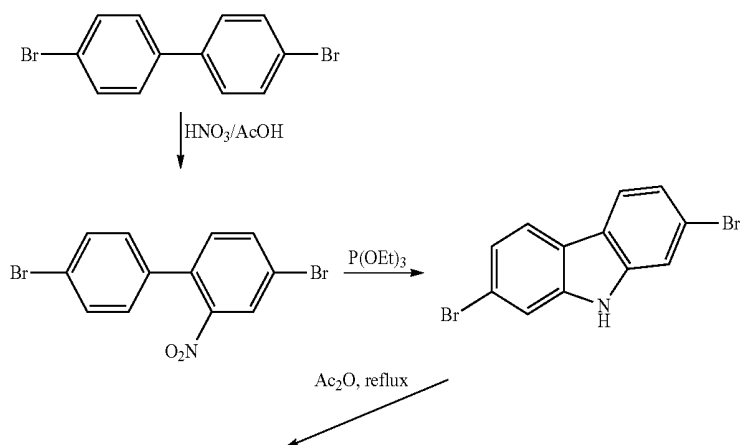
Scheme 6: Synthesis of compounds from 4-6 to 4-9
