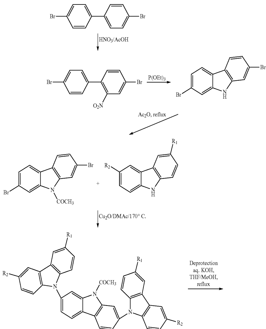
Scheme 5: Synthesis of compounds from 4-1 to 4-5
