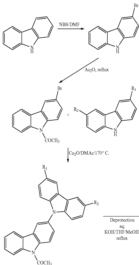
Scheme 2: Synthesis of compounds from 2-1 to 2-10
