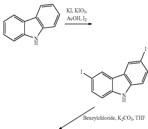
Scheme 11: Synthesis of compounds from 8-1 to 8-7
