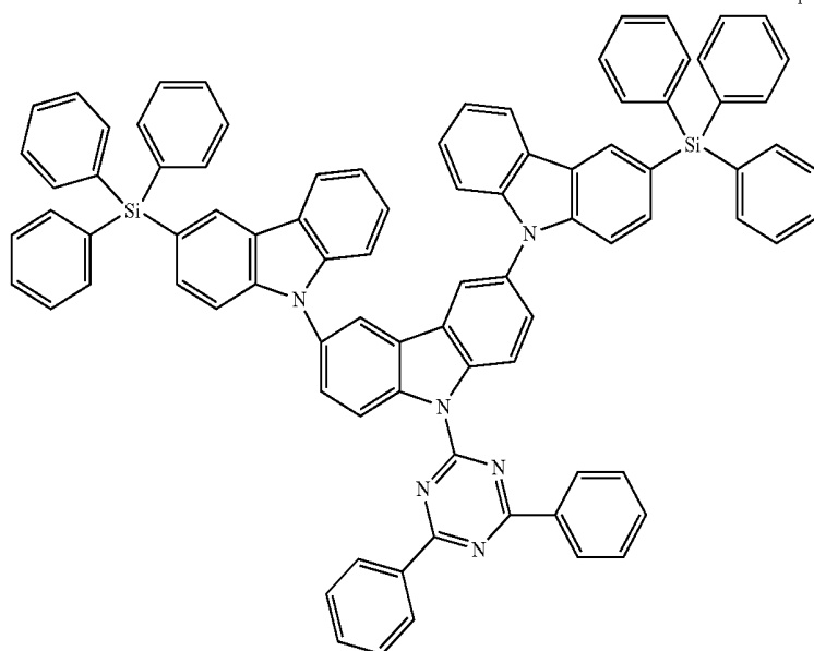
Compound 1-51
