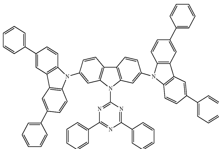
Compound 4-2
