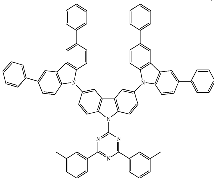
Compound 1-13
