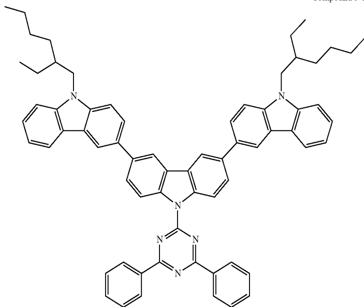
Compound 5-5
