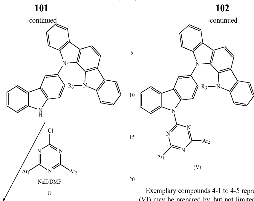
Scheme 5: Synthesis of compounds from 4-1 to 4-5
