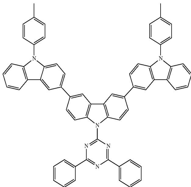
Compound 5-3
