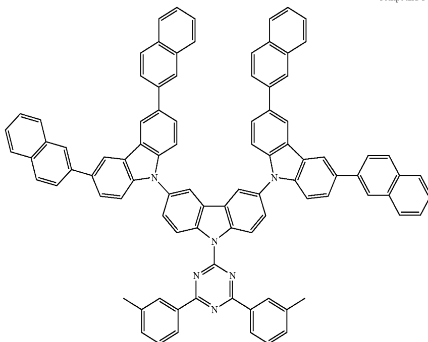
Compound 1-17
