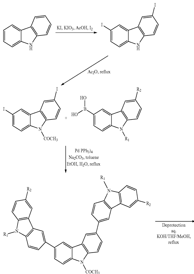
Scheme 7: Synthesis of compounds from 5-1 to 5-10
